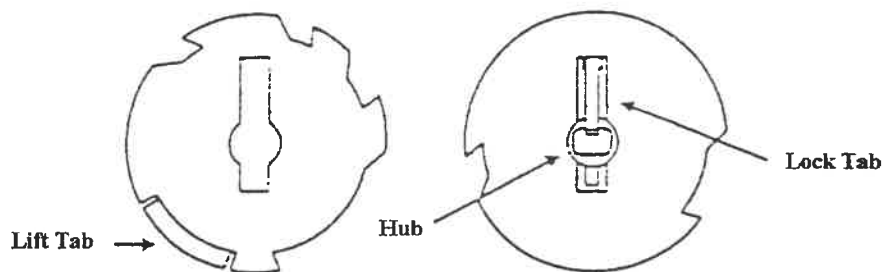
Fig. 5 Adjustable Cam
